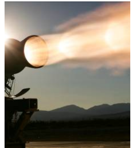
Test of Cooled Pintle Tip on Horizontal Test Stand
