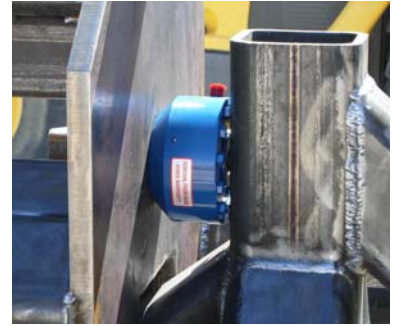
Thrust Load Cell
